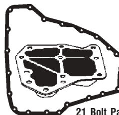
21 Bolt Pan RE4F04A FK82800B
